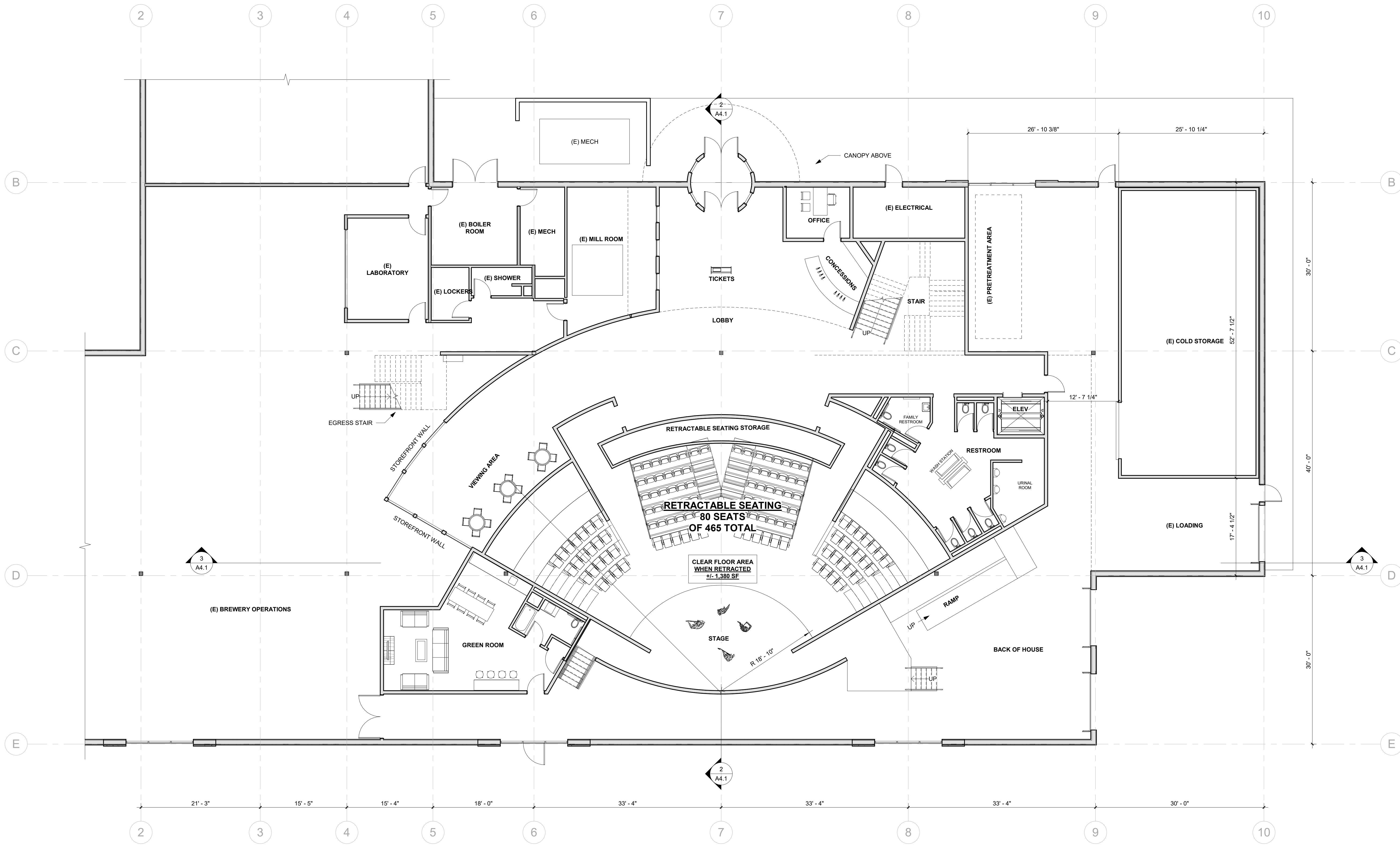
1 FLOOR PLAN - LEVEL 1 1/8" = 1'-0" @ FULL SIZE 0' 2' 4' 8'
