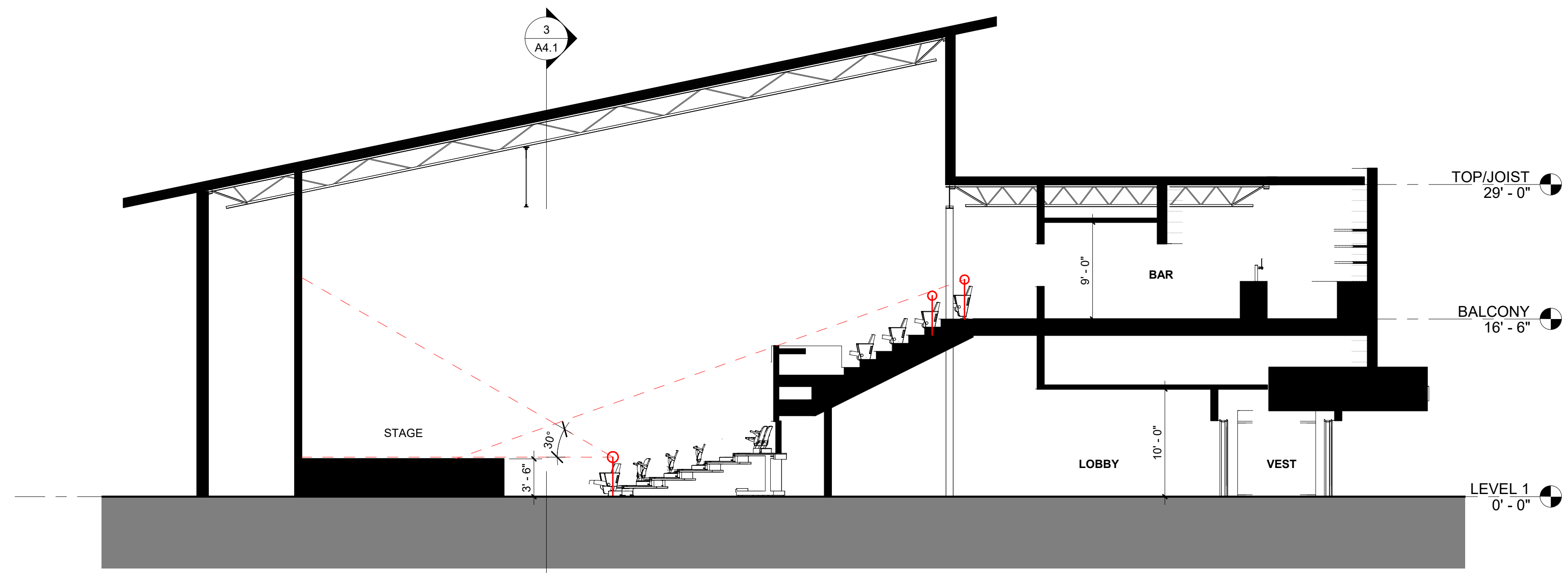
2 SECTION E/W 1/8" = 1'-0" @ FULL SIZE
