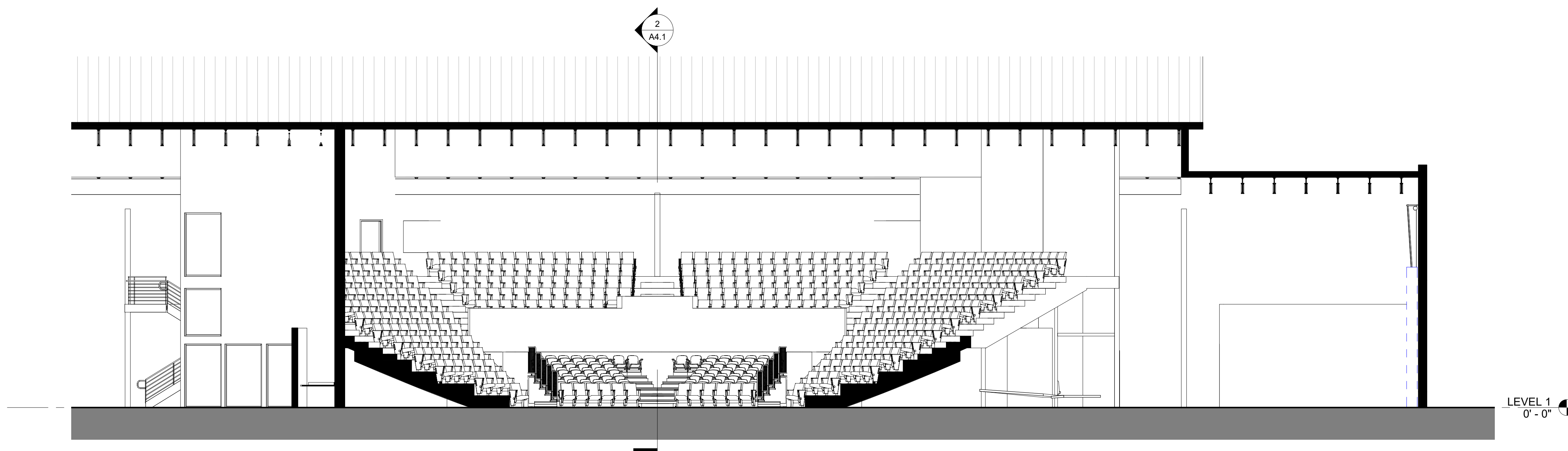
3 SECTION N/S 1/8" = 1'-0" @ FULL SIZE
